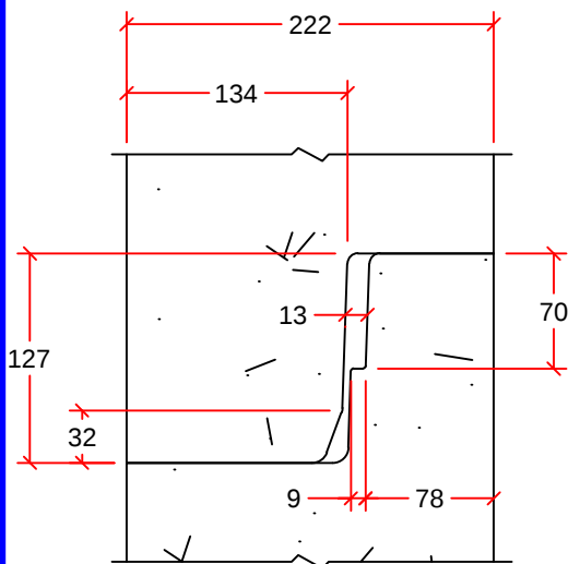
JOINT DETAIL
