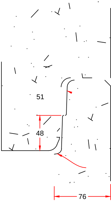
JOINT DETAIL
