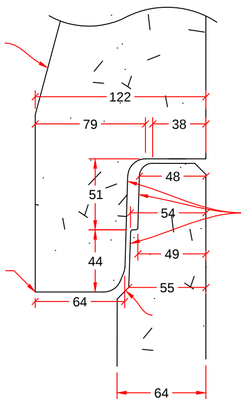
JOINT DETAIL
