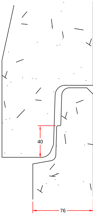
JOINT DETAIL
