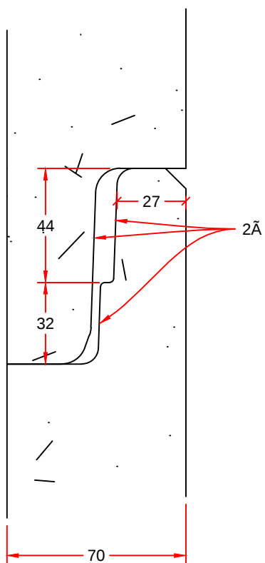
JOINT DETAIL
