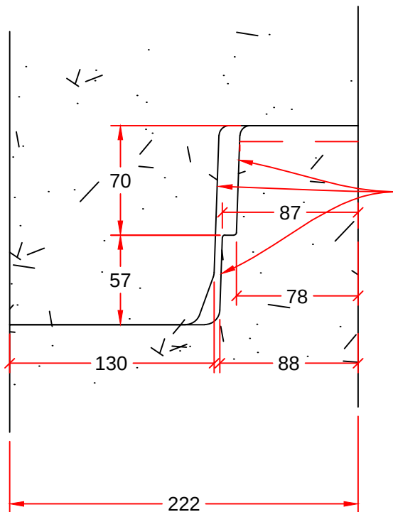
JOINT DETAIL
