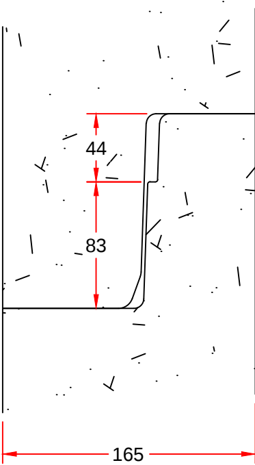
JOINT DETAIL
