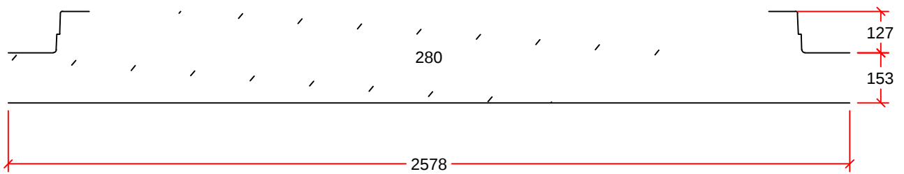
PROFILE VIEW
