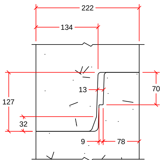
JOINT DETAIL
