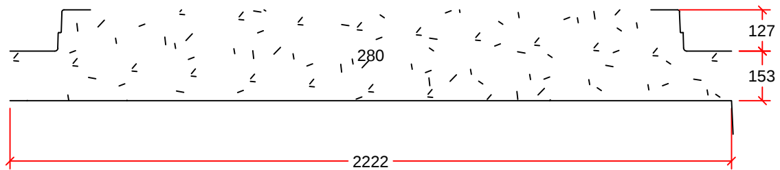
PROFILE VIEW
